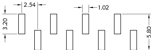
RECOMMENDED PCB LAYOUT (COMPONENT SIDE) (TOLERANCE: ±0.05)
